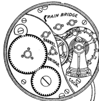
18 Size, 8th Model
