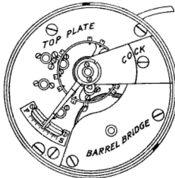
18 Size, 7th Model
