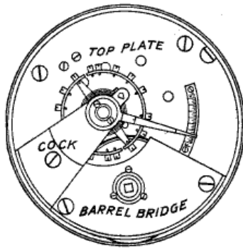
18 Size, 1st Model
