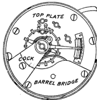
18 Size, 2d to 4th Model
