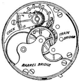
Hunting, Pendant Setting
