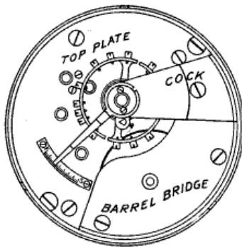
18 Size, 5th Model
